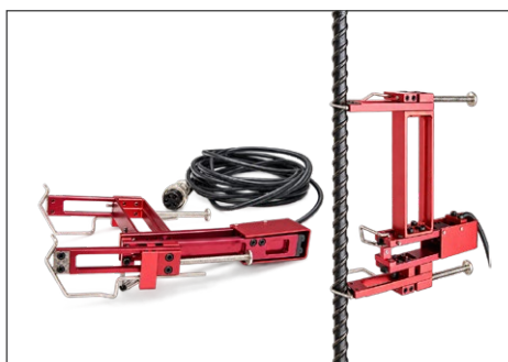
Axial Electronic Extensometer
